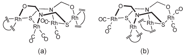
Figure 2. Possible C_2 isomers of compound [\text{Rh}_4(\mu\text{-PySO})_2(\text{cod})_2(\text{CO})_4] ( 5 ).
